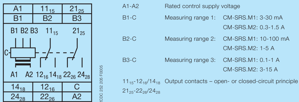
Connection diagram
