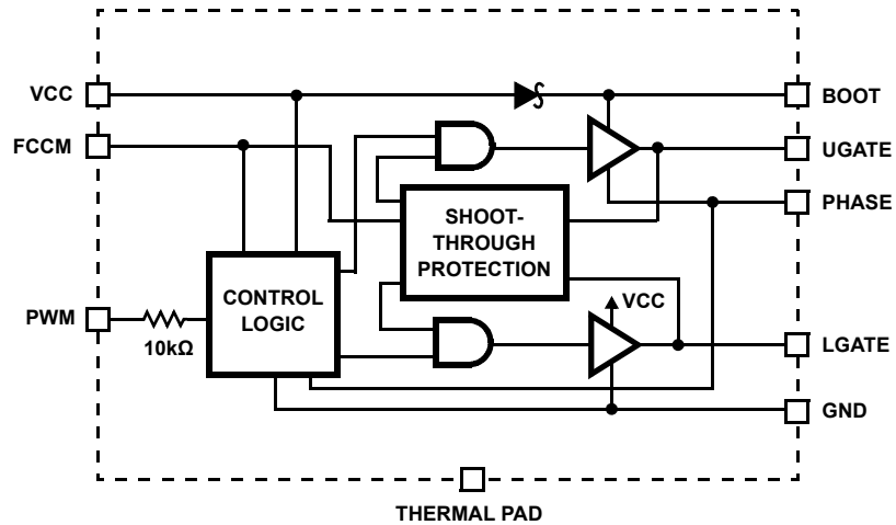
FIGURE 1. BLOCK DIAGRAM
