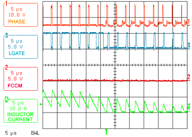
FIGURE 3. LOAD TRANSIENT (30A TO 0A, 3-PHASE)
