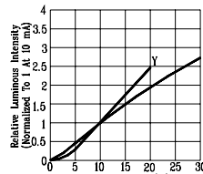
Fig6. RELATIVE LUMINOUS INTENSITY VS. FORWARD CURRENT
