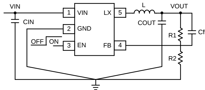
Figure 25. NCP1522 Board Schematic
