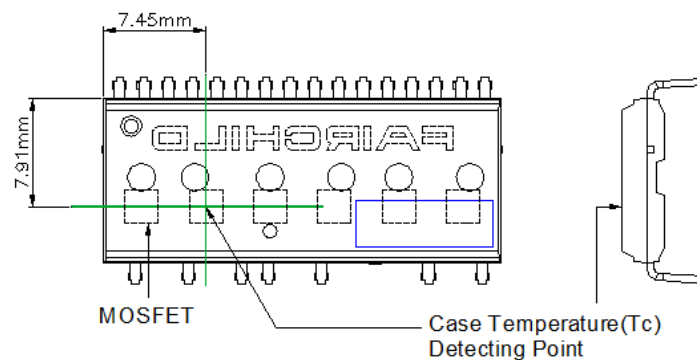
Figure 4. Case Temperature Measurement
