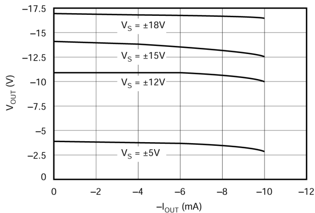
Figure 5-5. Maximum V_{\text{OUT}} vs I_{\text{OUT}} (Negative Swing)
