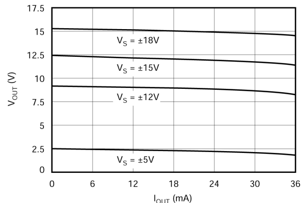
Figure 5-6. Maximum V_{\text{OUT}} vs I_{\text{OUT}} (Positive Swing)
