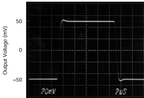
2μs/div Figure 5-3. Small-Signal Response ( R_{\text{LOAD}} = \infty , C_{\text{LOAD}} = 100\text{pF} )
