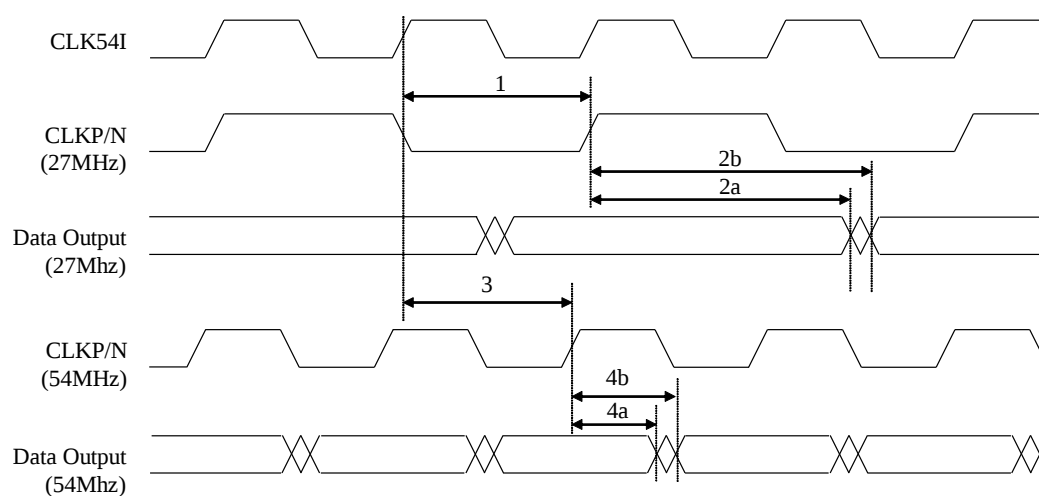
Fig19 CLK54I and Video Data Timing Diagram
