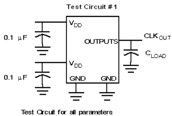
Figure 7. Test Circuits
