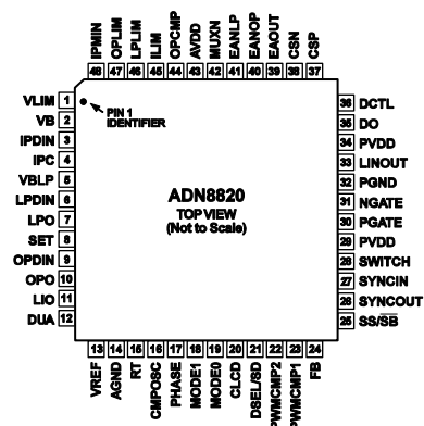
PIN CONFIGURATION
