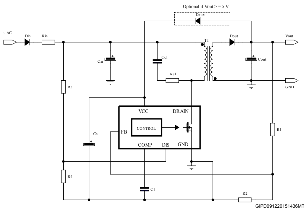
Figure 35. Flyback converter with line OVP (non-isolated)
