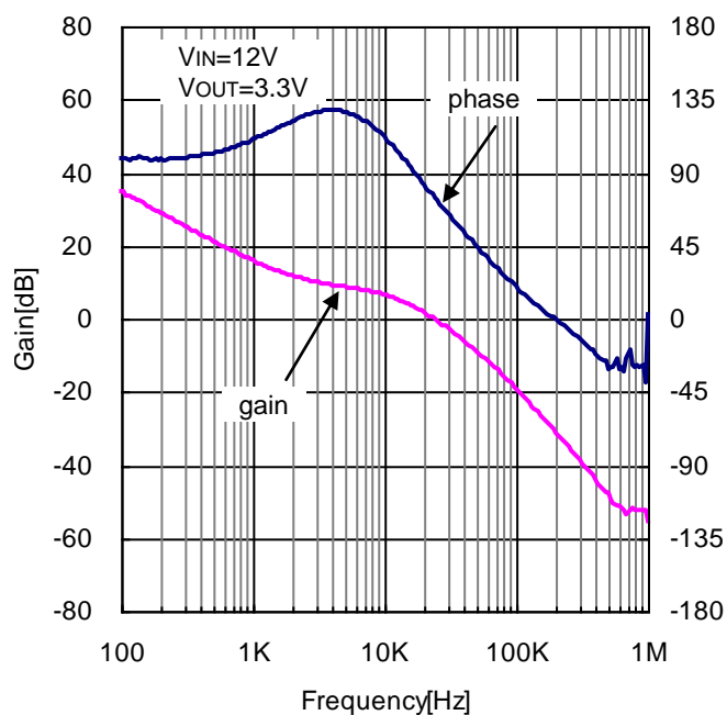
Figure 37. Loop Response (VIN=12V, VOUT=3.3V, IOUT=2.5A, COUT=Ceramic22 \mu F \times 2)
