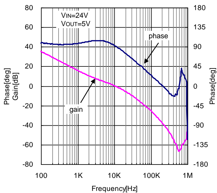
Figure 38. Loop Response (VIN=24V, VOUT=5V, IOUT=2.5A, COUT=Ceramic22 \mu F \times 2)
