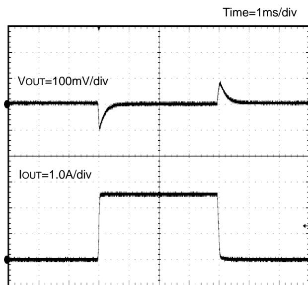
Figure 39. Load Transient Response IOUT=0A – 2.5A (VIN=12V, VOUT=3.3V, COUT=Ceramic22 \mu F \times 2)
