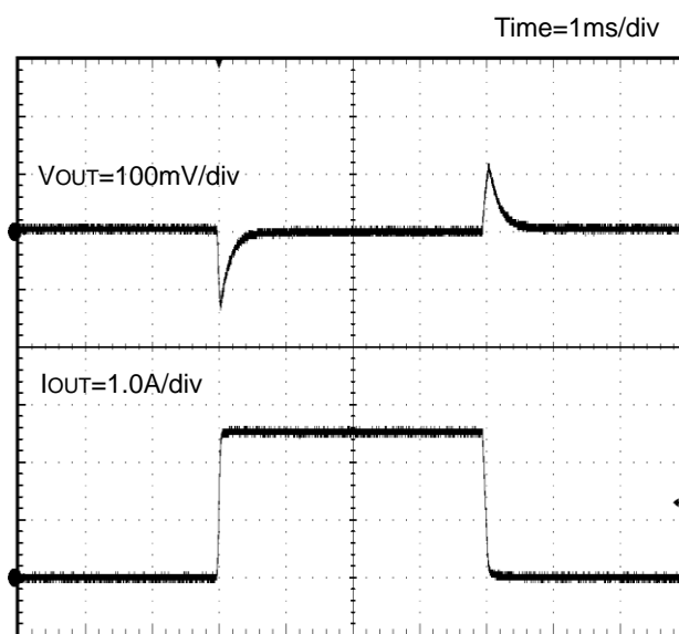
Figure 40. Load Transient Response IOUT=0A – 2.5A (VIN=24V, VOUT=5.0V, COUT=Ceramic22 \mu F \times 2)
