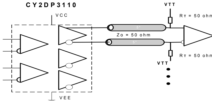
Figure 7. Standard LVPECL – PECL Output Termination
