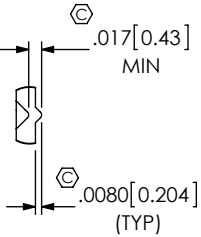
CRIMP DETAIL SCALE: 4:1 (TYP ALL CRIMPS)
