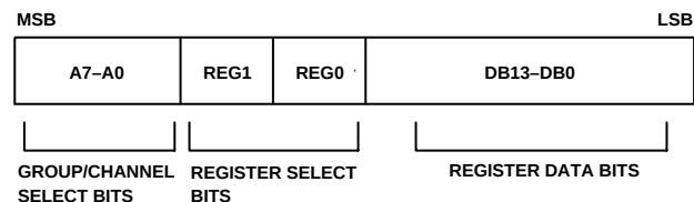
Figure 21. Serial Data Format
