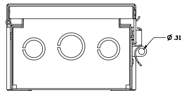
BOTTOM VIEW
