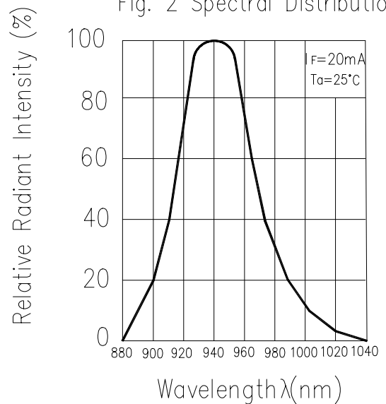
Fig. 2 Spectral Distribution
