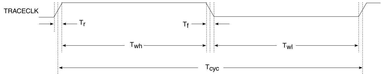
Figure 5. TRACE_CLKOUT specifications
