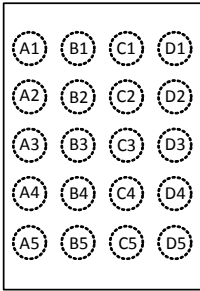
ISL91108 (20 BUMP WLCSP) TOP VIEW
