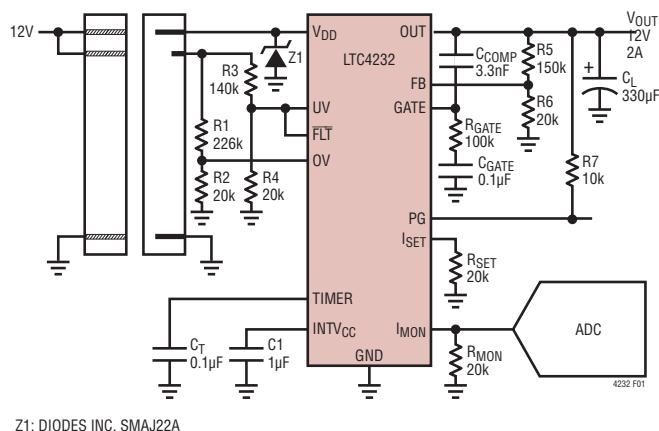
Figure 1. 2A, 12V Card Resident Application
