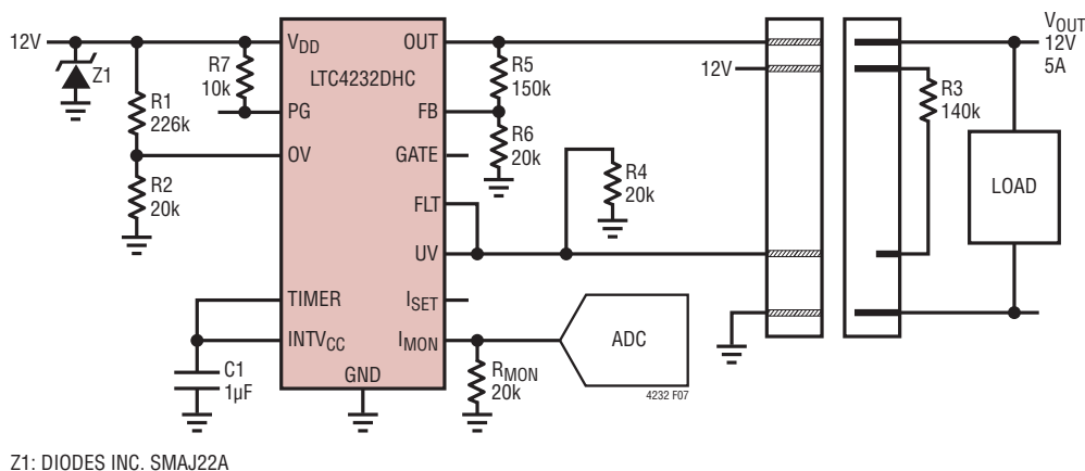
Figure 7. 12V, 5A Backplane Resident Application with Insertion Activated Turn-On
