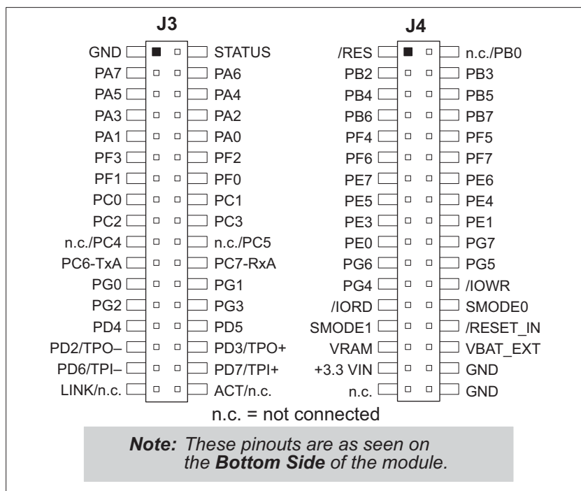
Figure 5. RCM3360/RCM3370 Pinouts
