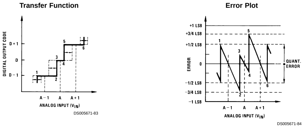
FIGURE 2. Clarifying the Error Specs of an A/D Converter Accuracy= \pm \frac{1}{4} LSB
