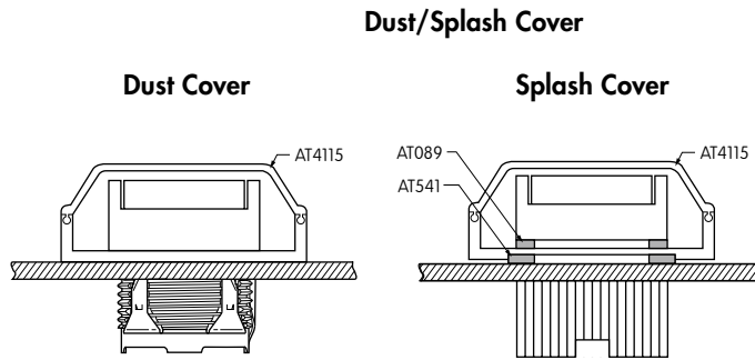
Snap-in Mount
