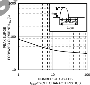
I_{FSM} CYCLE CHARACTERISTICS
