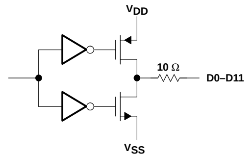
Figure 5. Digital Outputs
