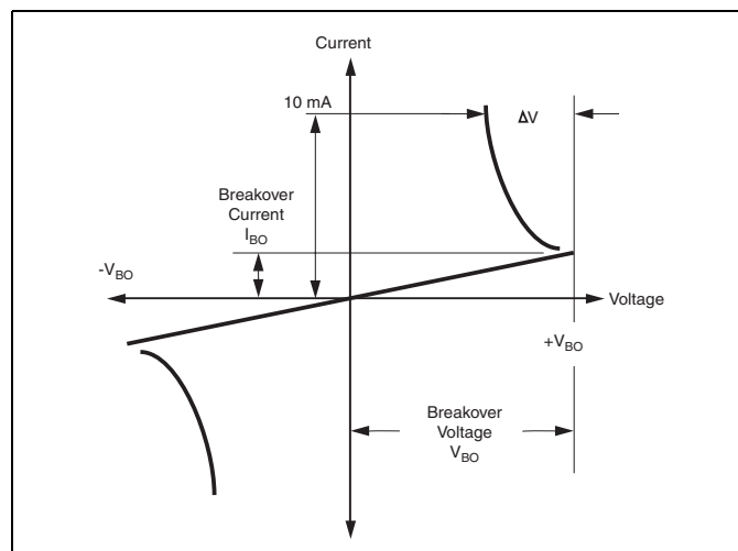
V-I Characteristics
