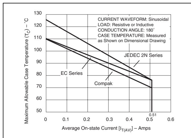
Figure E5.3 Maximum Allowable Case Temperature versus Average On-state Current
