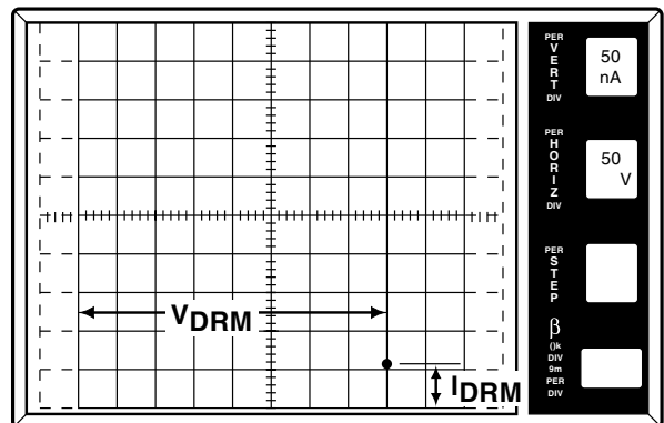
Figure AN1006.18 (+)I_{DRM} = 51 \text{ nA} at (+)V_{DRM} = 400 \text{ V}
