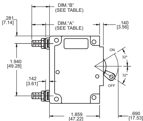
Single Pole
