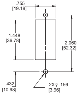
Mounting Detail
