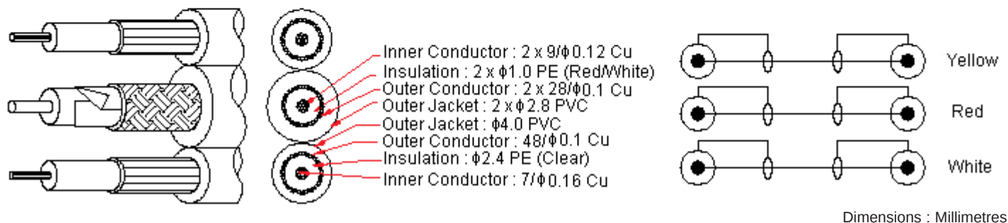
Wiring Diagram
