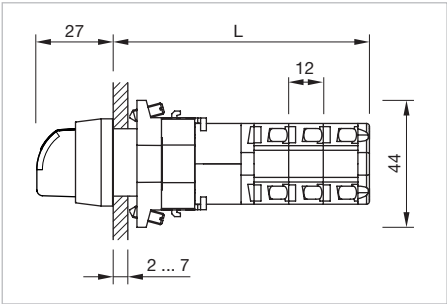
Dimensions [mm] L = (Number of stages x 12) + 54.5 mm
