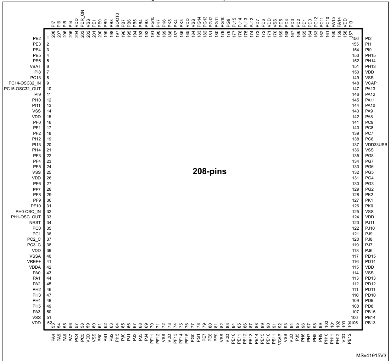
Figure 11. LQFP208 pinout
