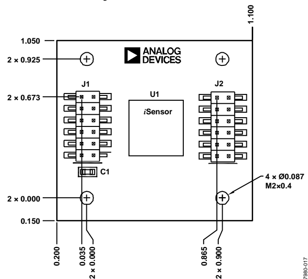
Figure 18. PCB Assembly View and Dimensions
