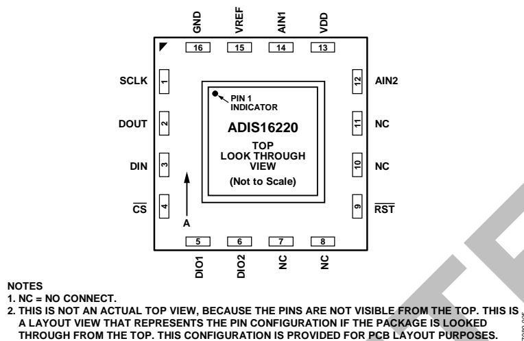
Figure 4. Pin Configuration
