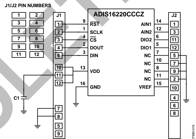
Figure 17. Electrical Schematic
