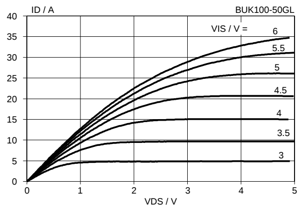
Fig.7. Typical on-state characteristics, T_j = 25^\circ\text{C} . I_D = f(V_{DS}) ; parameter V_{IS} ; t_p = 250\text{ }\mu\text{s}
