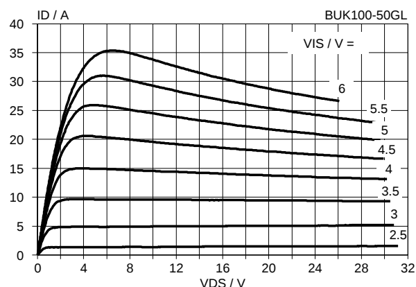
Fig.6. Typical output characteristics, T_j = 25^\circ\text{C} . I_D = f(V_{DS}) ; parameter V_{IS} ; t_p = 250\text{ }\mu\text{s} & t_p < t_{dsc}
