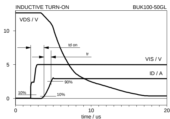
Fig.24. Typical switching waveforms, inductive load. V_{DD} = 13 \text{ V} ; I_D = 3 \text{ A} ; R_I = 50 \Omega ; T_j = 25 \text{ }^\circ\text{C} .
