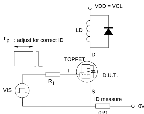
Fig.23. Test circuit for inductive load switching times.
