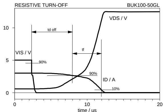
Fig.22. Typical switching waveforms, resistive load. V_{DD} = 13 \text{ V} ; R_L = 4 \Omega ; R_I = 50 \Omega ; T_j = 25 \text{ }^\circ\text{C} .
