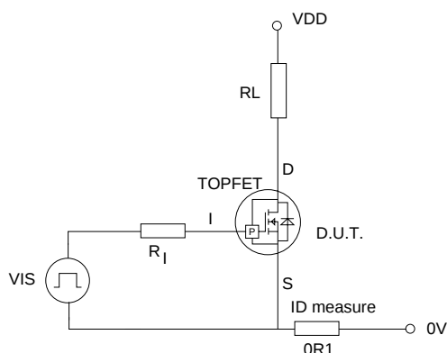
Fig.20. Test circuit for resistive load switching times.
