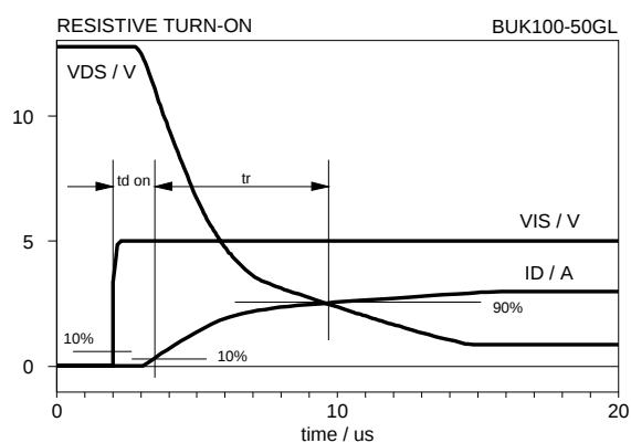
Fig.21. Typical switching waveforms, resistive load. V_{DD} = 13 \text{ V} ; R_L = 4 \Omega ; R_I = 50 \Omega ; T_j = 25 \text{ }^\circ\text{C} .
