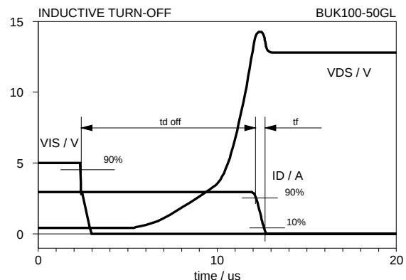
Fig.25. Typical switching waveforms, inductive load. V_{DD} = 13 \text{ V} ; I_D = 3 \text{ A} ; R_I = 50 \Omega ; T_j = 25 \text{ }^\circ\text{C} .
