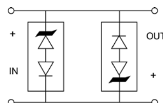
FIGURE 4 Optional Bidirectional configuration (two TVS devices in anti-parallel)
