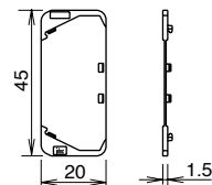
HW-VG1 Dual Pushbutton Barrier
