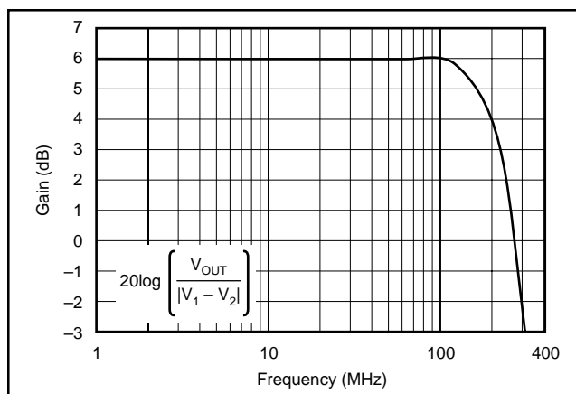
FIGURE 4. High-Speed Instrumentation Amplifier Response.
