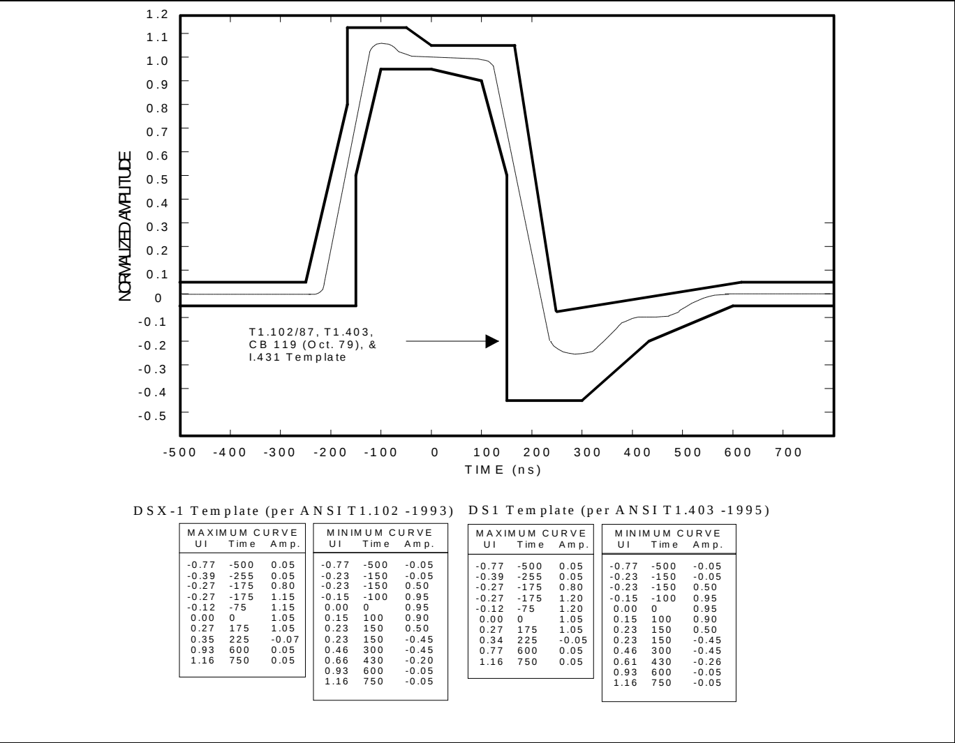
Figure 5-6. T1 Transmit Pulse Templates
