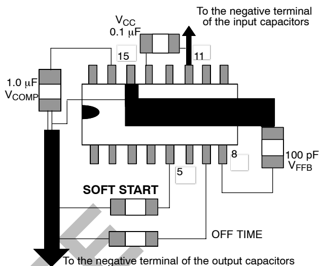
Figure 23. Layout Guidelines
