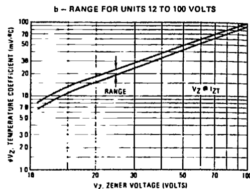
Figure 4 TEMPERATURE COEFFICIENTS
