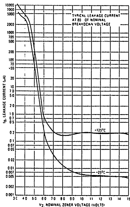
Figure 3 TYPICAL LEAKAGE CURRENT
