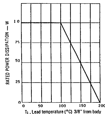
Figure 2 POWER DERATING
