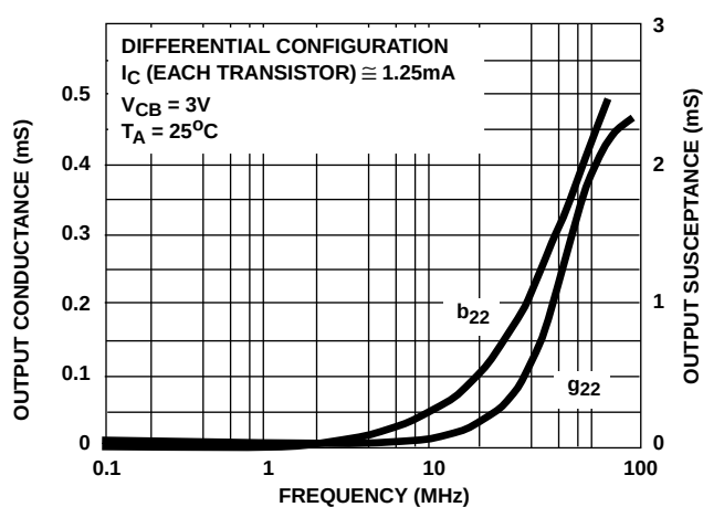
FIGURE 17. OUTPUT ADMITTANCE ( Y_{22} ) vs FREQUENCY
