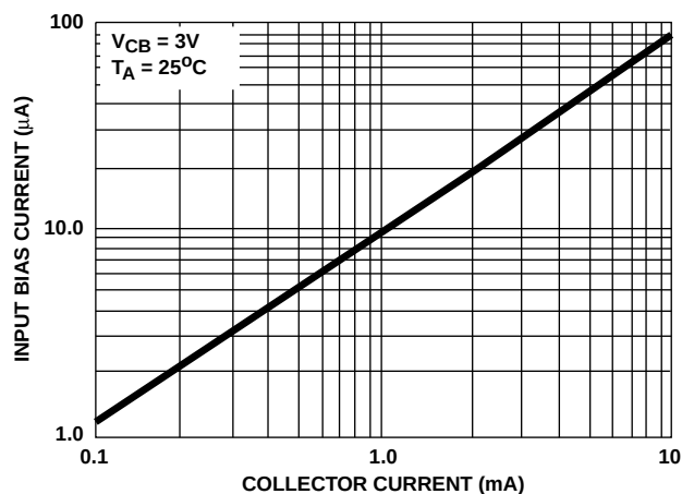
FIGURE 5. INPUT BIAS CURRENT vs COLLECTOR CURRENT FOR EACH TRANSISTOR
