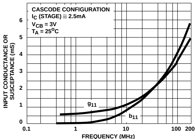
FIGURE 20. INPUT ADMITTANCE ( Y_{11} ) vs FREQUENCY
