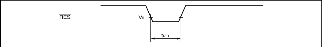
Figure 17.2 \overline{\text{RES}} Low Width Timing
