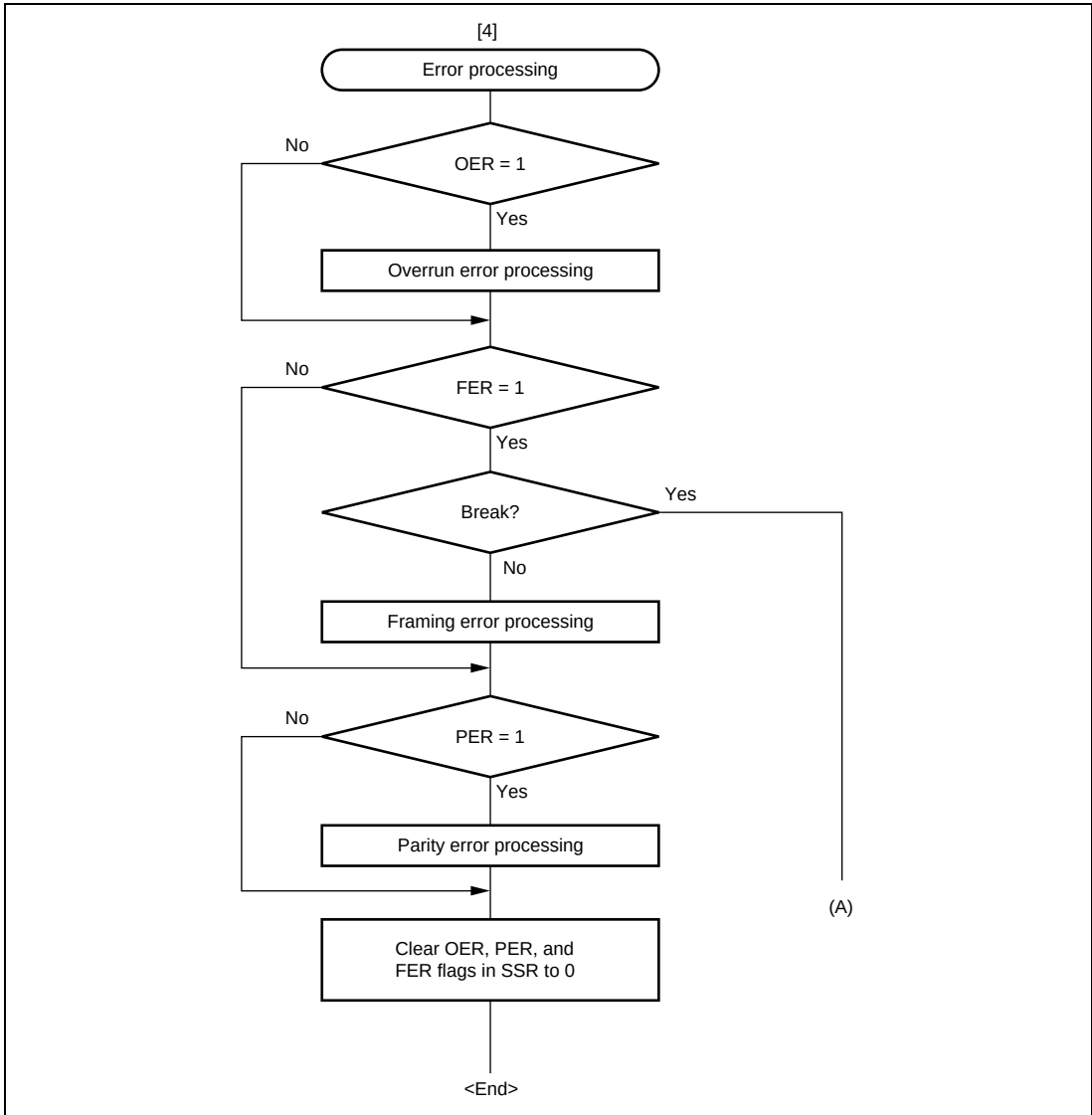
Figure 10.8 Sample Serial Data Reception Flowchart (Asynchronous Mode) (2)
