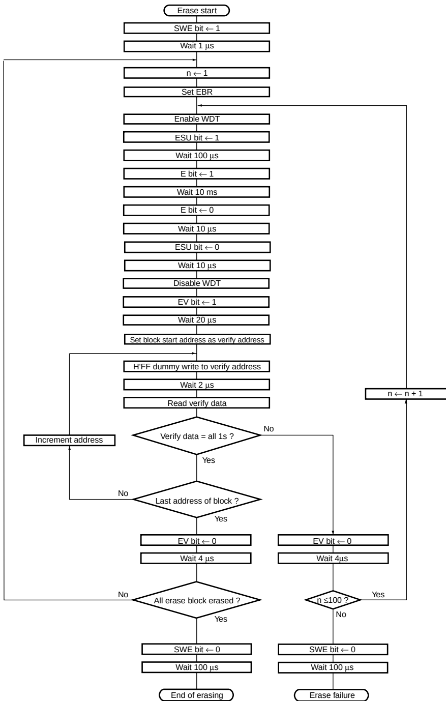
Figure 6.11 Erase/Erase-Verify Flowchart
