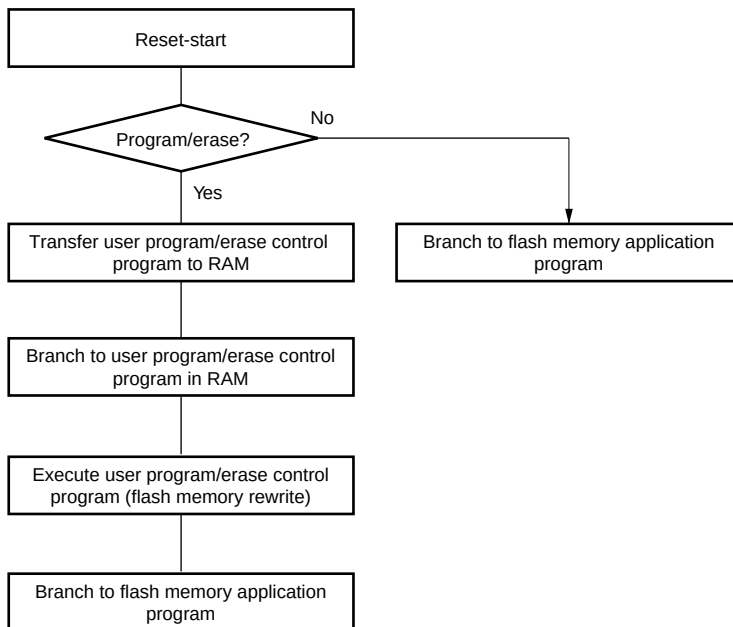
Figure 6.9 Programming/Erasing Flowchart Example in User Program Mode
