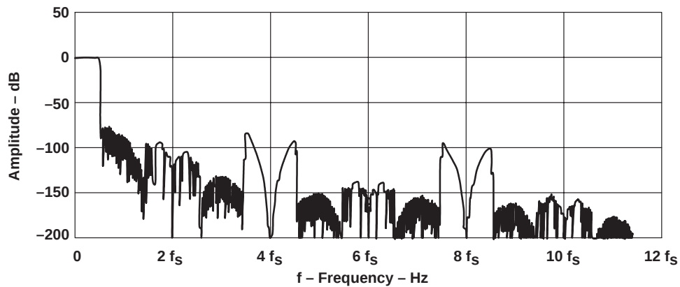
Figure 4-6. ADC Digital Filter Characteristics
