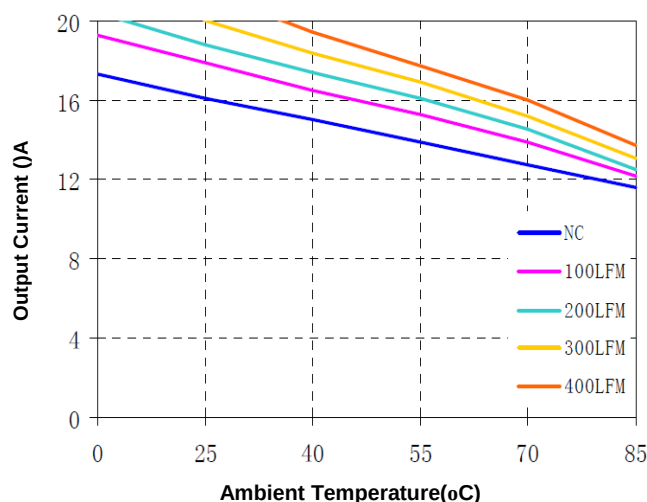
Figure 12(f). Current Derating Curve for 5V Output ( V_{in} = 12V open frame)
