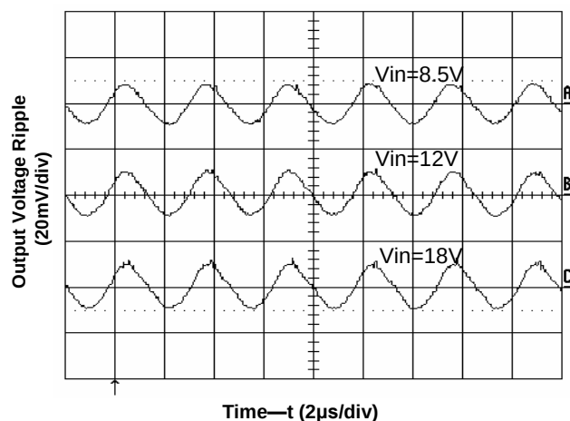
Figure 2. Output Voltage Ripple at 2.5V, 20A Output
