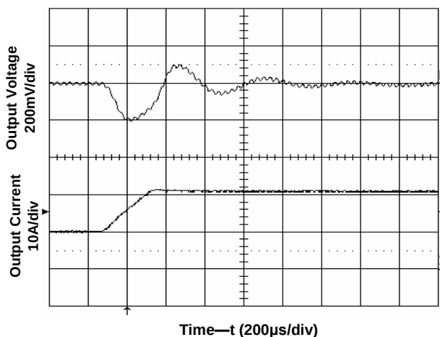
Figure 9. Transient Load Response Input voltage 12V, Output current 10A -> 20A, Slew rate 0.5A/μs
