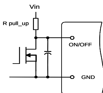
Fig. 14 Circuit for Negative Logic Control
