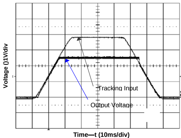
Figure 11. Voltage Tracking/Sequencing (with tracking option) Vin= 12V, Vo = 2.5V, Io = 0A
