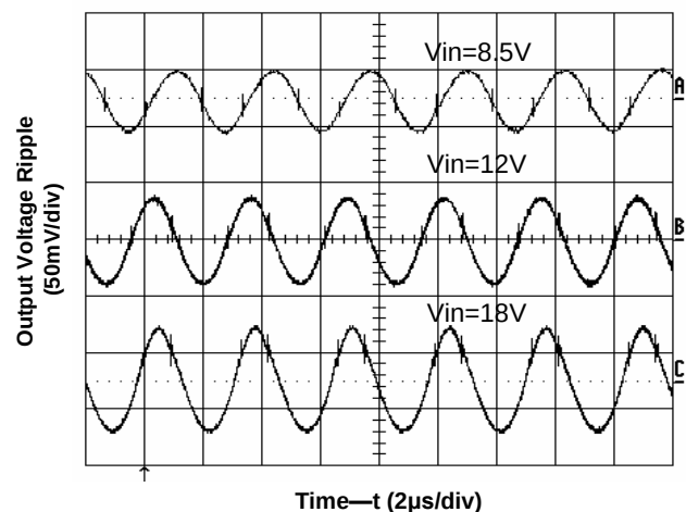
Figure 3. Output Voltage Ripple at 5V, 20A Output
