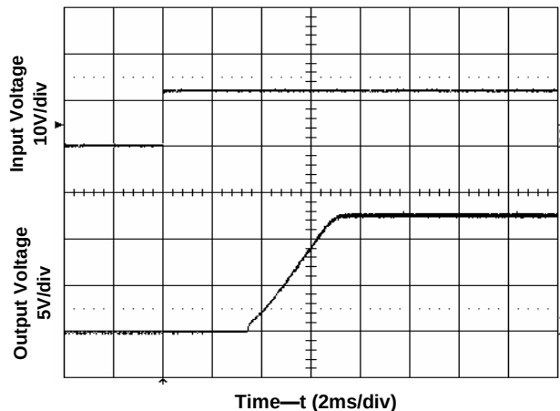
Figure 5. Start-up Application of Input Voltage Input voltage 12V, Output current 0A
