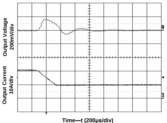
Figure 8. Transient Load Response Input voltage 12V, Output current 20A->10A, Slew rate 0.5A/μs.
