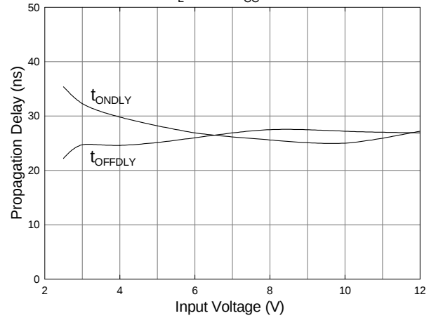
Fig. 18 Propagation Delay vs. Input Voltage C_L=15\text{nF} V_{CC}=15\text{V}
