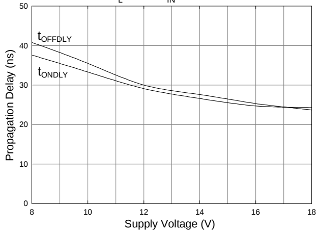
Fig. 17 Propagation Delay vs. Supply Voltage C_L=15\text{nF} V_{IN}=5\text{V@1kHz}
