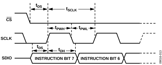
Figure 40. Timing Diagram for Serial Port Register Write ( t_{DS} to t_{DCS} )
