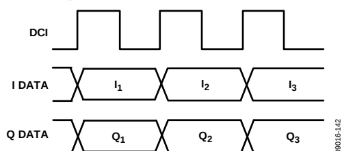
Figure 42. Timing Diagram for Dual-Word Mode
