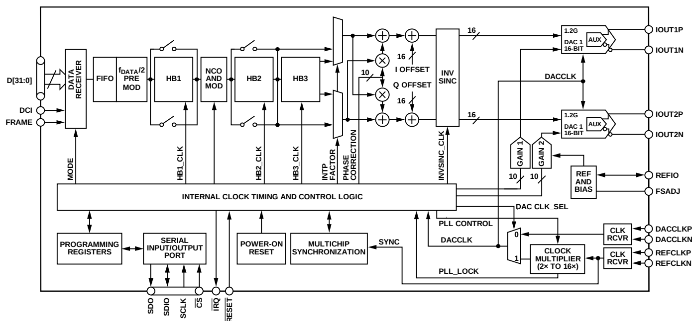
Figure 2. AD9125 Functional Block Diagram
