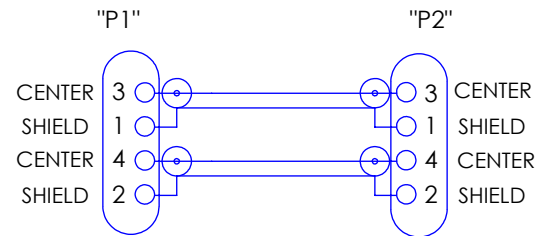
WIRING DIAGRAM
