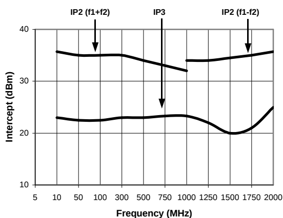
Intermodulation Intercept
