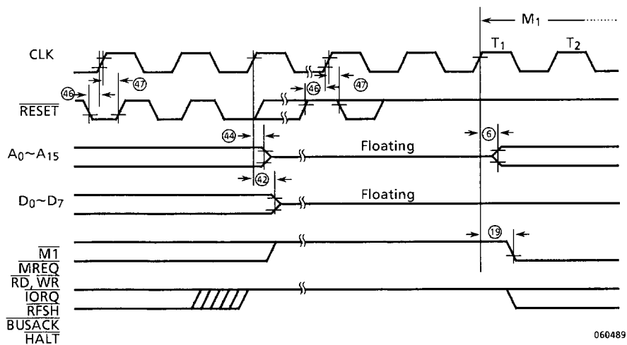
Figure 4.8 Reset Cycle
