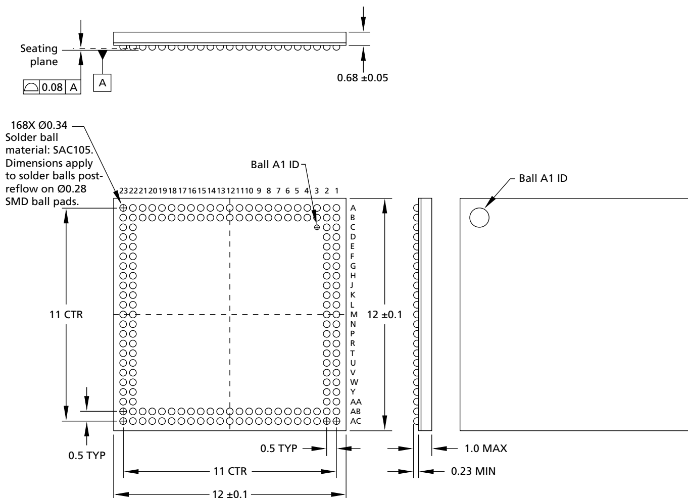
Figure 13: 168-Ball VFBGA (12mm x 12mm), Package Code: JV
