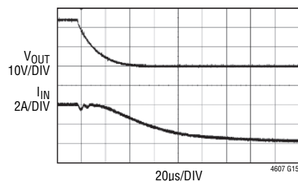
Short-Circuit with 36V IN to 24V OUT at I OUT = 6A
