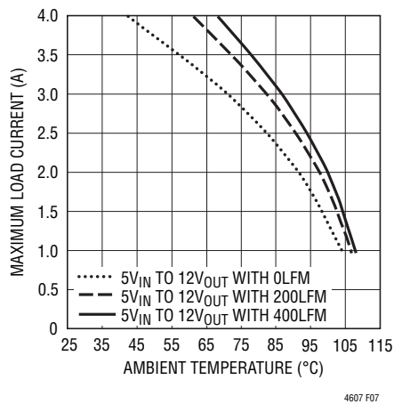
Figure 7. 5V IN to 12V OUT without Heat Sink
