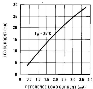
LED Current vs Referenced Loading
