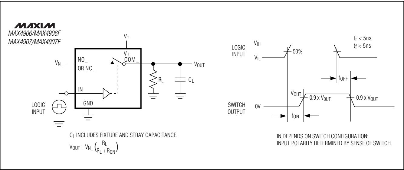
Figure 3. Switching Time
