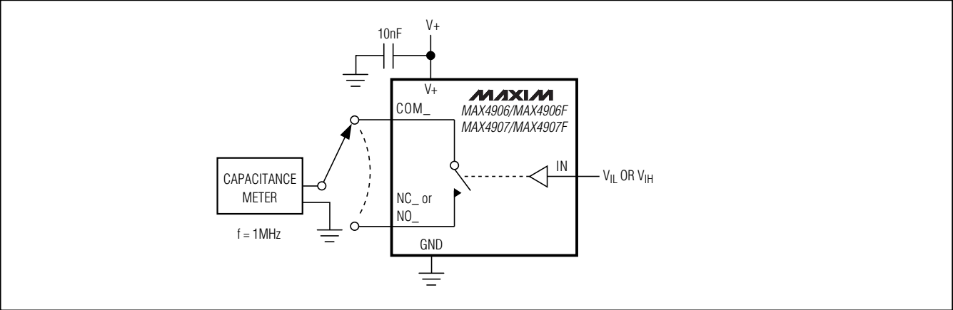
Figure 2. Channel Off/On-Capacitance
